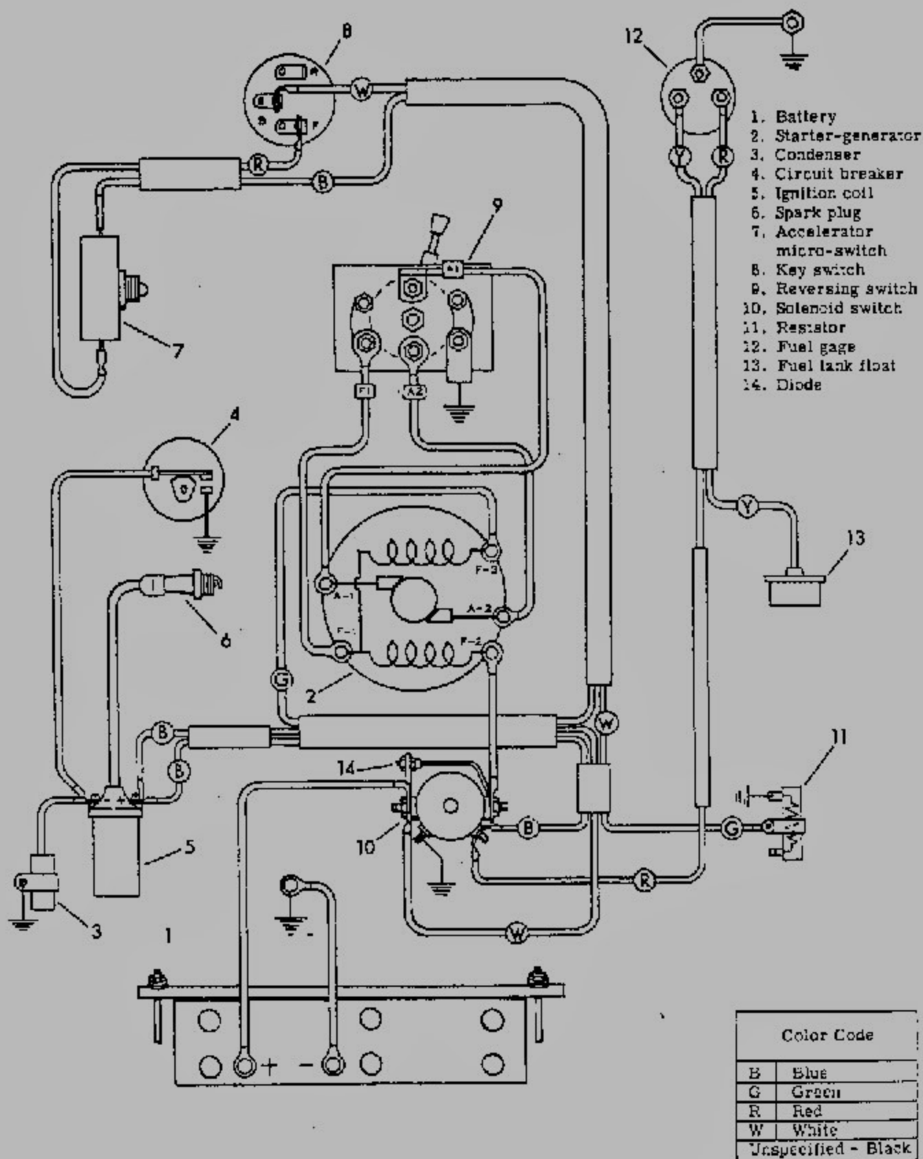
Figure 5B-24. 1957 - Early 1968 Model D Wiring Diagram
