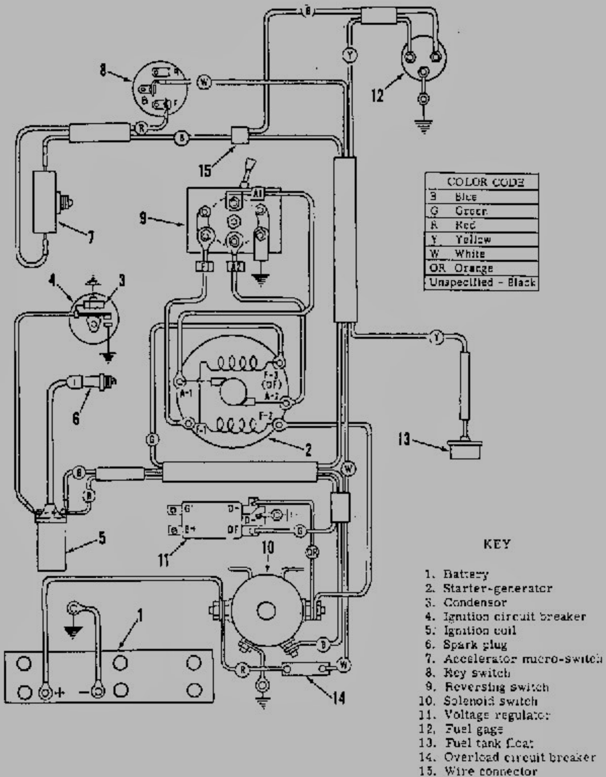
Figure 5B-25. Late 1966 to Early 1972 Model D Wiring Diagram
