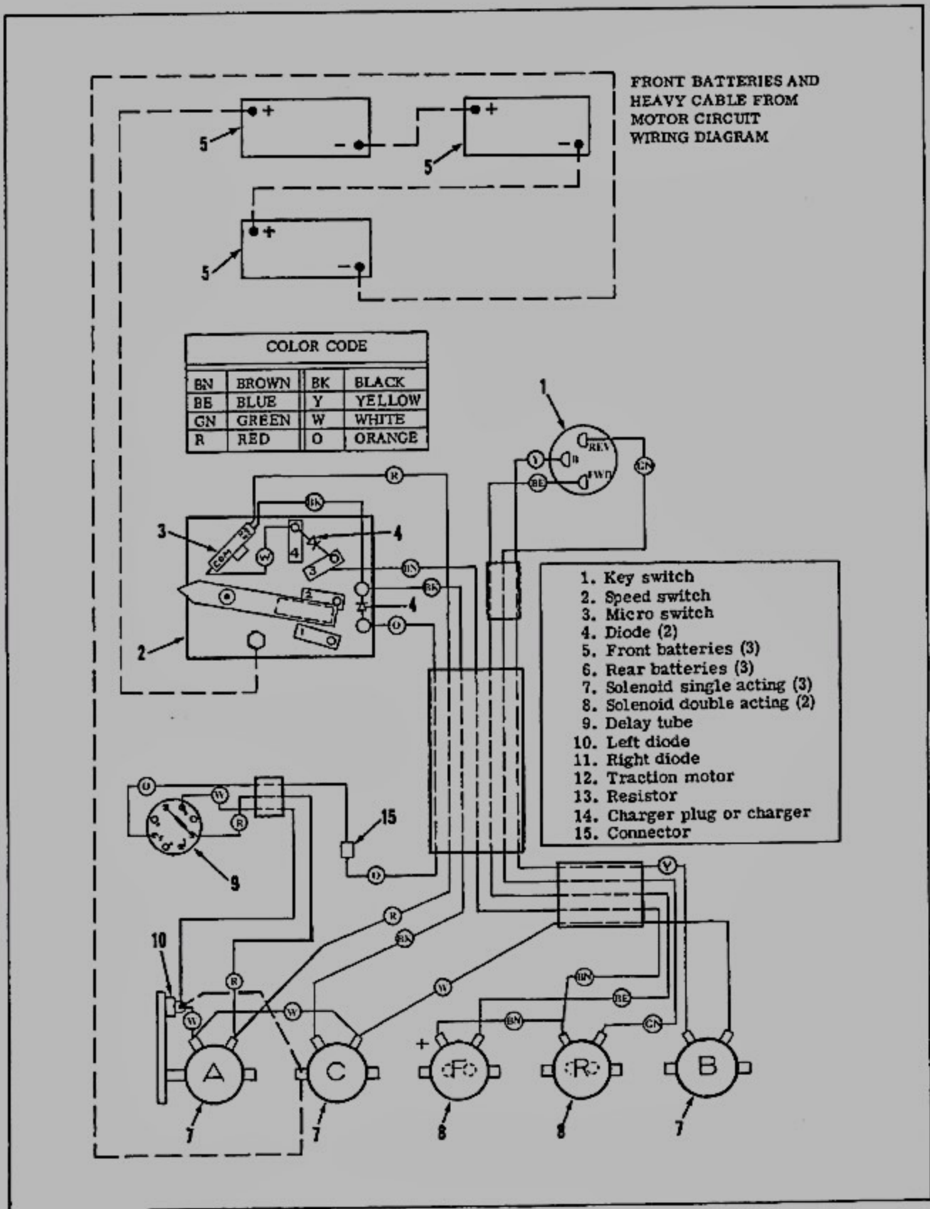
Figure 5-31. 1972-1975 Model DE and DE-4 Wiring Diagram - 16 Gage Wire Control Circuit
