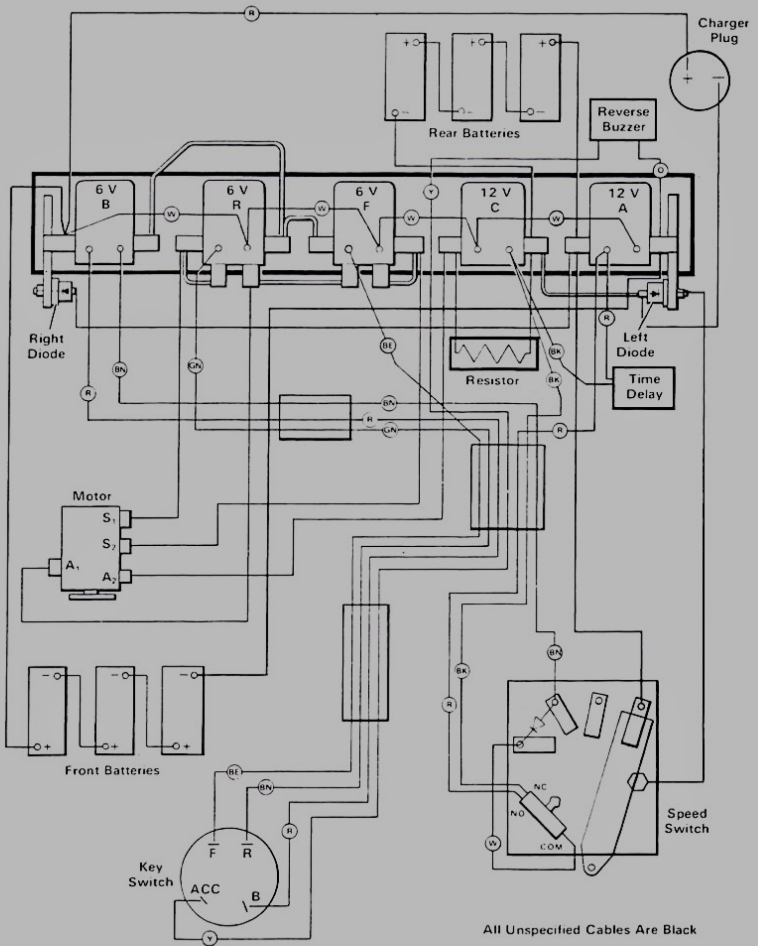
WIRING DIAGRAM 1979-1982
