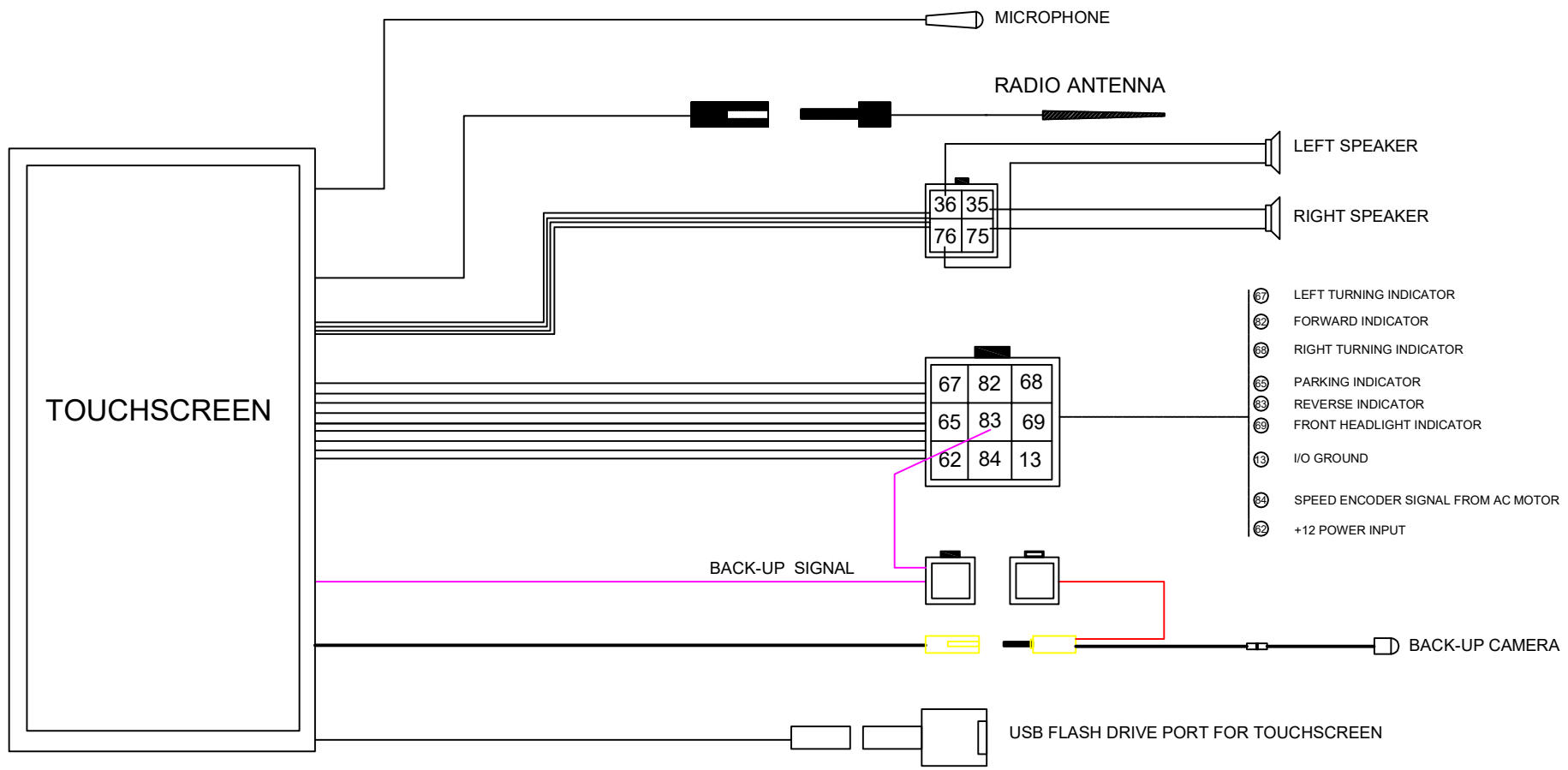
TOUCHSCREEN WIRING DIAGRAM
