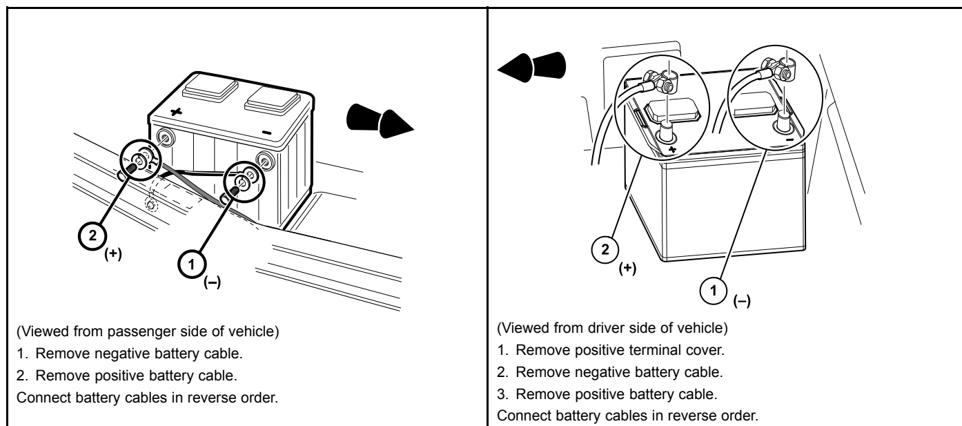
3167 Figure 4 Top-Post Battery Cable Removal: Gasoline Vehicles
