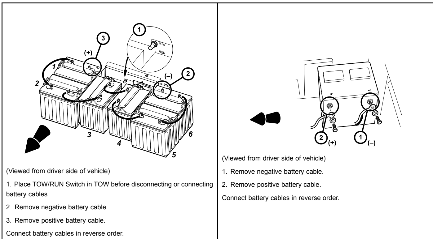
Figure 2 Battery Cable Removal – 6x8-Volt Battery Configuration
