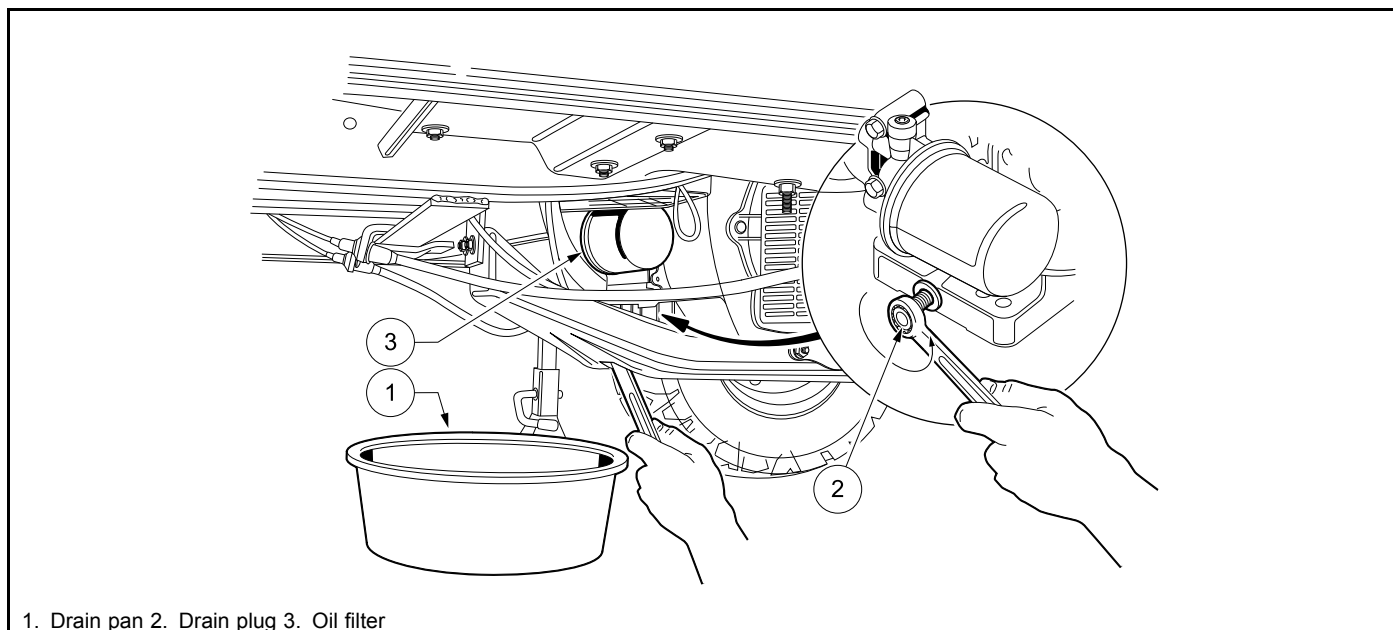
25 Figure 37 Engine Oil Drain Plug and Pan
