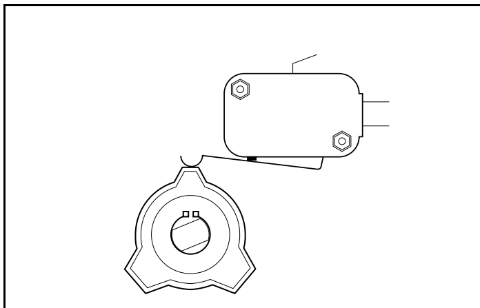
Figure 20 Neutral Lockout – Maintenance Position
