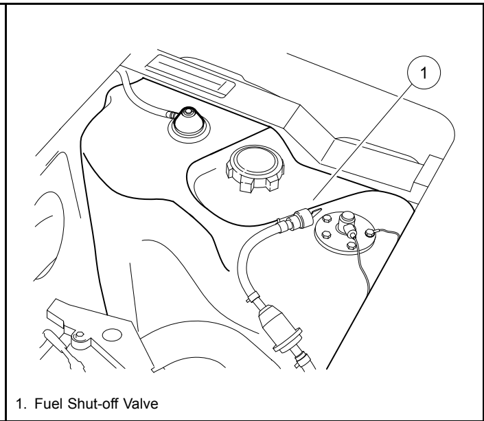
Figure 25 Fuel Tank
