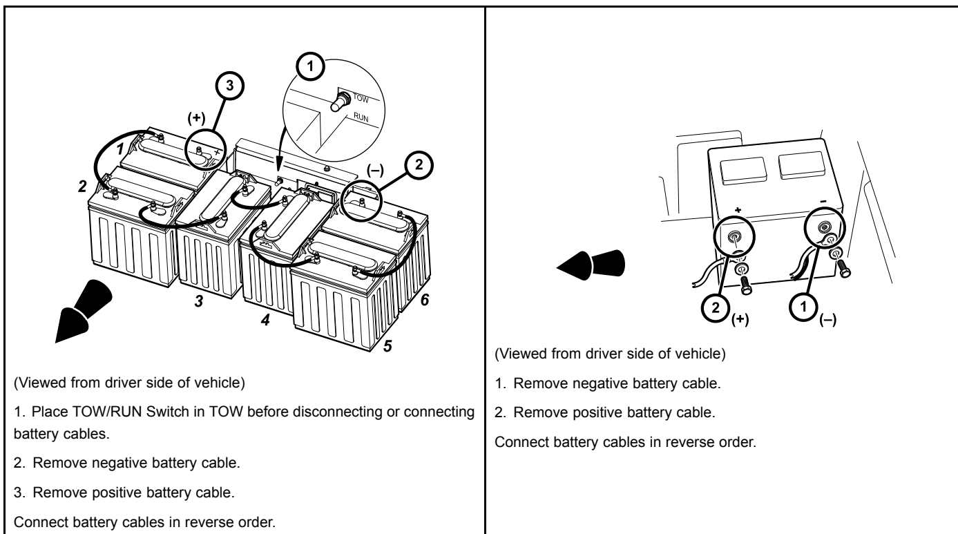
49A Figure 3 Battery Cable Removal – 6x8-Volt Battery Configuration
