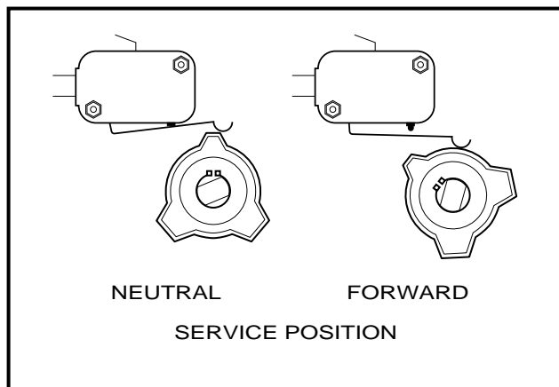
Figure 8 Neutral Lock-out – Service
