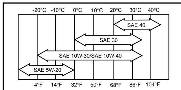
Figure 18 Oil Viscosity
