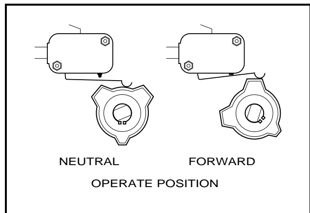
Figure 9 Neutral Lock-out – Operate
